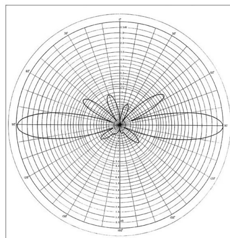
F23H Radiation Pattern E-Plane
