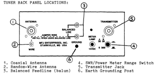
TUNER BACK PANEL LOCATIONS:
