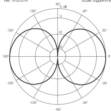
TYPICAL RADIATION PATTERN in E-plane at mid-band File: E-02-074 Scale: logarithmic
