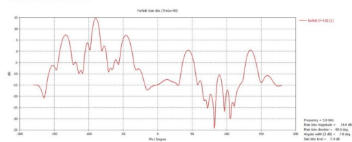
H-Plane Radiation Pattern
