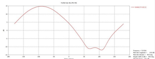
H-Plane Radiation Pattern
