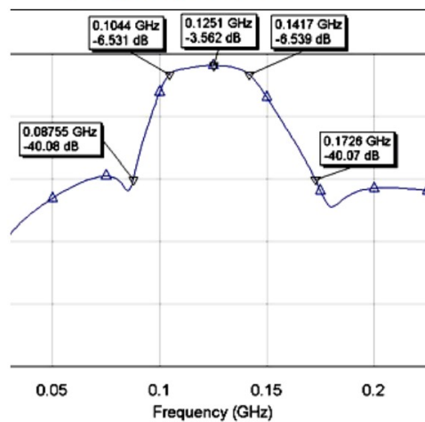
ABF128 Frequency Response
