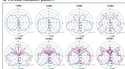
■ Vertical radiation pattern
