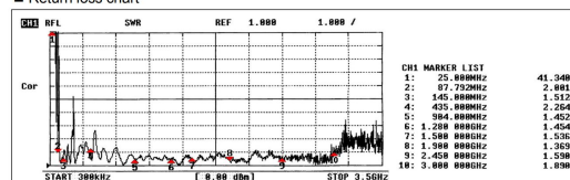
■ Return loss chart
