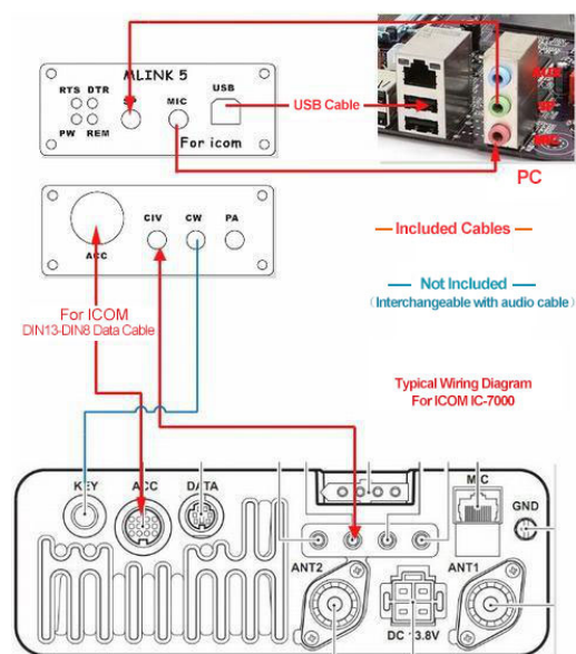
Wiring diagram For ICOM IC-703, 706, 706MK2, 706MK2G, 718, 78, 7000, 7200, etc., for example, connection to IC-7000.
