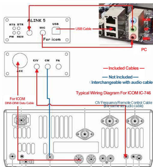
Connection diagram for ICOM IC-707, M710, 725, 725A, 726, 728, 729, 735, 736, 737, 738, 746, 746PRO, 756, 756PRO, 756PRO2, 756PRO3, 761, 775, 781, 910, 7400, 7600, 7800 and the like. For example, connection to IC-746.
