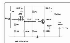
Circuit diagram of the padWh-Mini-Whip.
