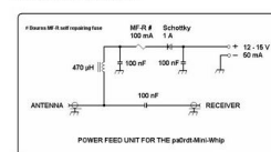
Power Feed Unit circuit diagram.
