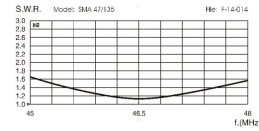
TYPICAL S.W.R. RESPONSE
