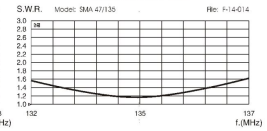
TYPICAL S.W.R. RESPONSE
