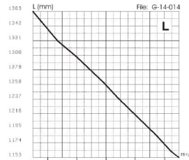
TYPICAL TUNING DIAGRAM vs FREQUENCY
