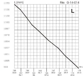
TYPICAL TUNING DIAGRAM vs FREQUENCY
