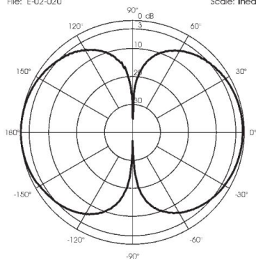
TYPICAL RADIATION PATTERN in E-plane at 122 MHz File: F-02-020 Scale: linear
