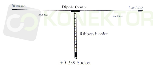
G5RV Antenna - 1/2 Size
